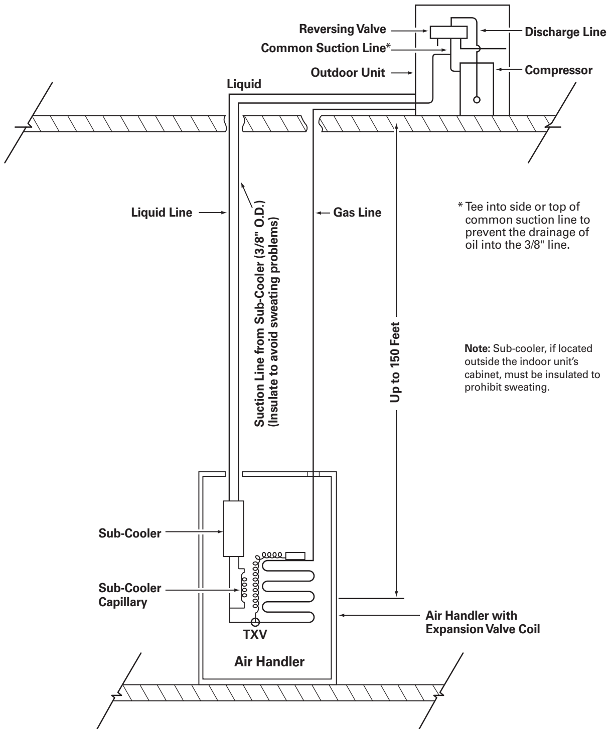
Figure 5 High Lift Heat Pump Piping Schematic (Outdoor Unit above Air Handler)
